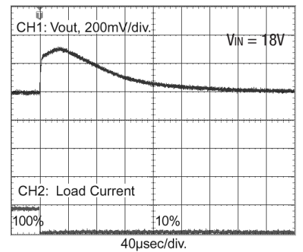
7803SR 100% to 10% Load Step
