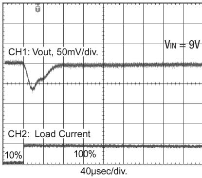
7803SR 10% to 100% Load Step
