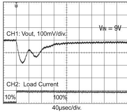
7805SR 10% to 100% Load Step
