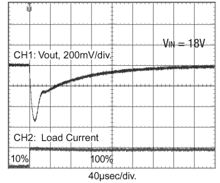
7812SR 10% to 100% Load Step
