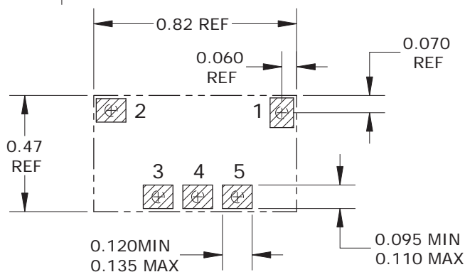
Figure 2. OKY-T/3, -T/5 Mechanical Outline
