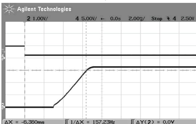
On/Off Enable Startup Delay (Vin=12V, Vout=3.3V, Iout=0.04A, Load=0) Trace 4=Enable In, Trace2=Vout
