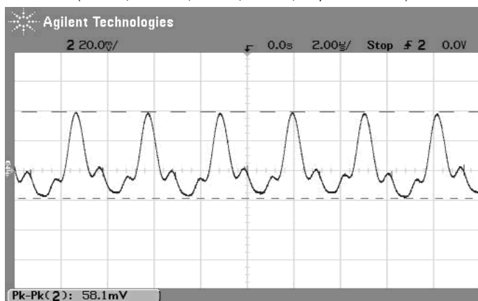
Output Ripple and Noise (Vin=12V, Vout=3.3V, Iout=3A, Load=0, ScopeBW=100MHz)
