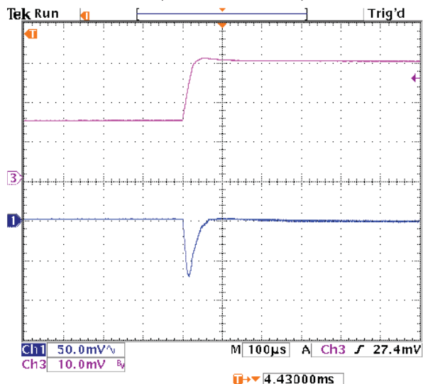
Step Load Transient Response (Vin=12V, Vout=3.3V, Load=0, Iout=1.5A to 3A) Trace 1=Vout, 50 mV/div. Trace 3=Iout, 1A/div.
