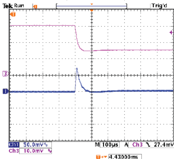
Step Load Transient Response (Vin=12V, Vout=3.3V, Load=0, Iout=3A to 1.5A) Trace 1=Vout, 50 mV/div. Trace 3=Iout, 1A/div.
